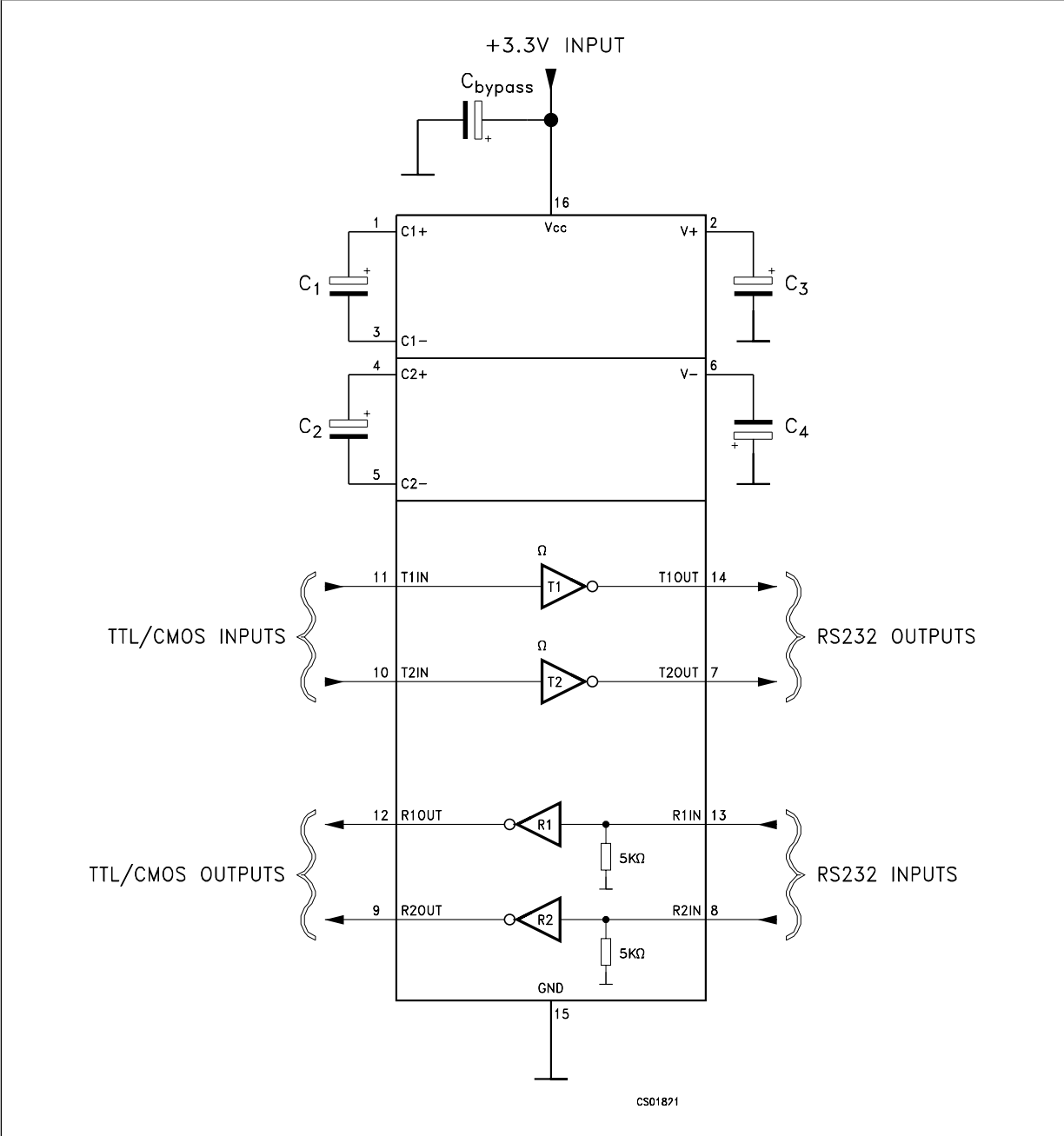
Figure 2. Application circuits
